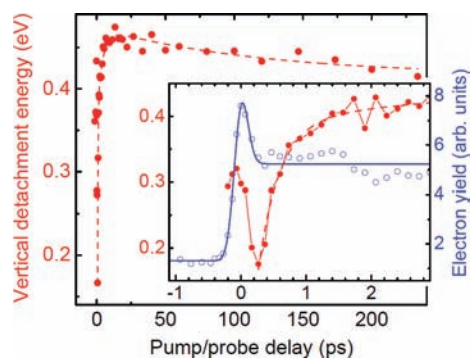
FIGURE 11. Extracted VDE (red circles) and excited-state detachment yield (blue circles) from time-dependent spectra of \text{I}^-(\text{CH}_3\text{CN})_5 in Figure 10. 57
