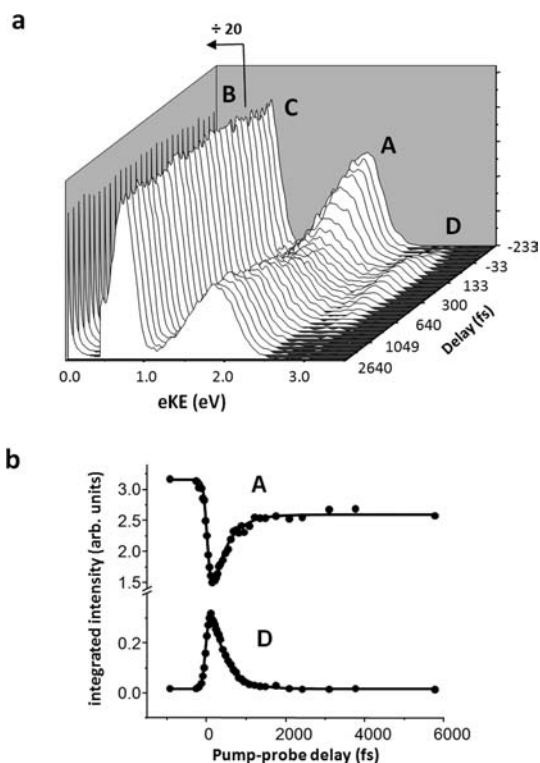
FIGURE 6. (a) Time-resolved photoelectron spectra of water cluster anions (D_2O)_{25}^- at pump and probe photon energies of 1.0 and 3.1 eV, respectively. (b) Integrated photoelectron intensities of ground- and excited-state detachment features A and D.
